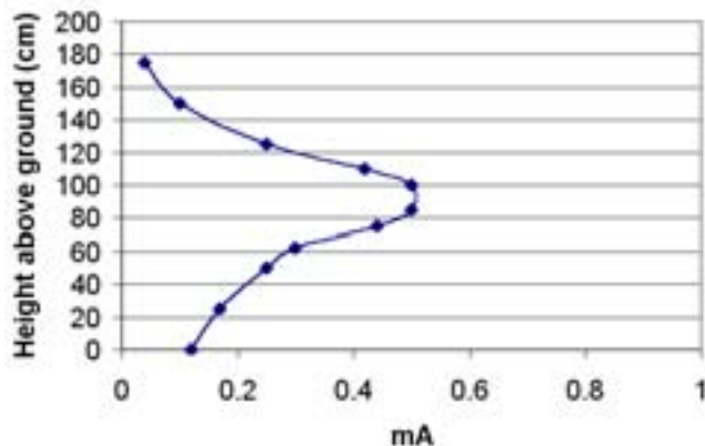
Figure 17. Induced vertical1 current distribution for isolated, shoe-wearing, grounded or ground-topped human model at 27.12 MHz under near-field exposure conditions. 16
