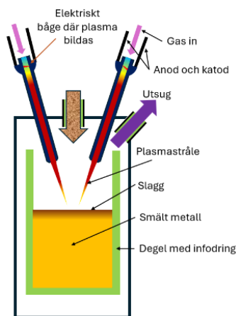
Figur 393: Plasmaugn i genomskärning.
