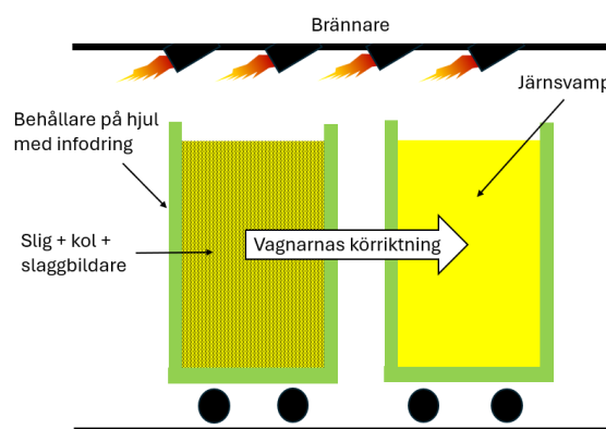
Figur 19: Principskiss tunnelugn.
