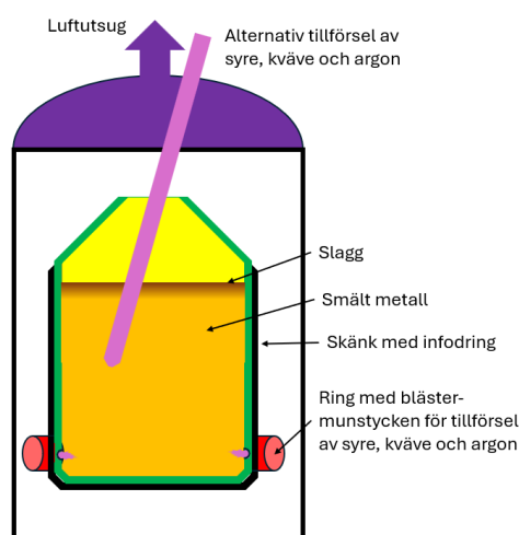
Figur 25: AOD-konverter i genomskärning.
